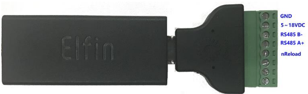
Figure 8. EW11+8PIN Connector
